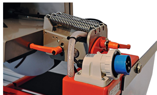
Monophasé, triple ressort
