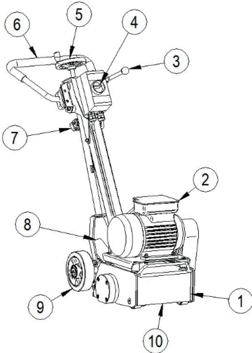
Functional machine parts SCARIMAX 200
