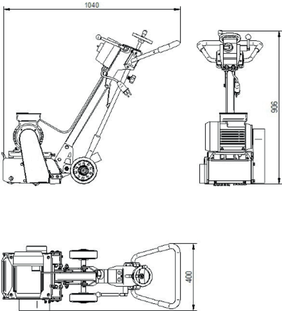
Machine dimensions SCARIMAX 200
